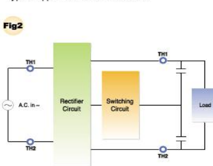
Typical application of ICL in SMPSU
