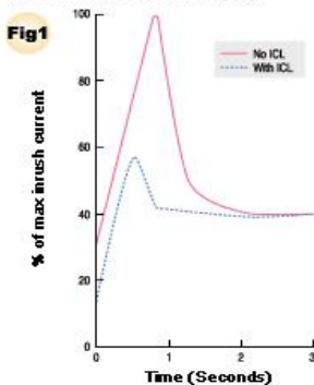
Typical ICL effect on Inrush Current in Switch Mode power supply
