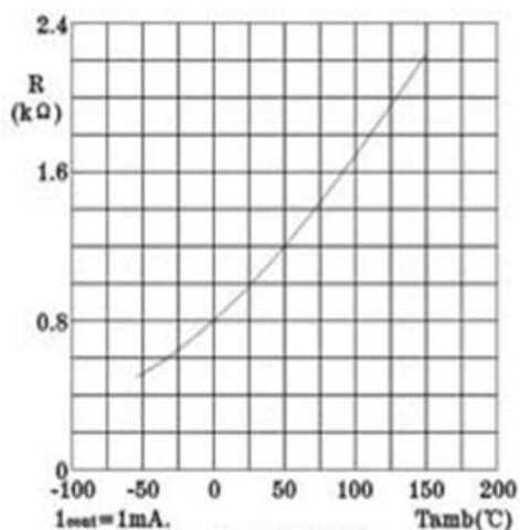
KTY81 Series
