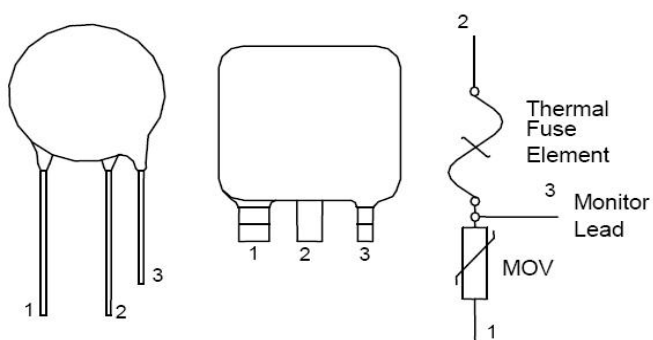
Three-terminal(3A/3B Type)
