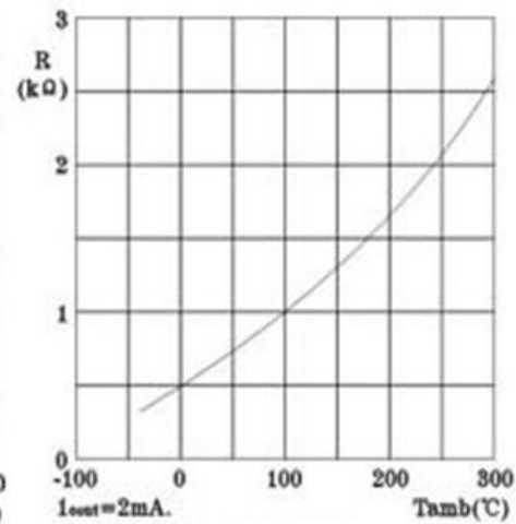
KTY84 Series
