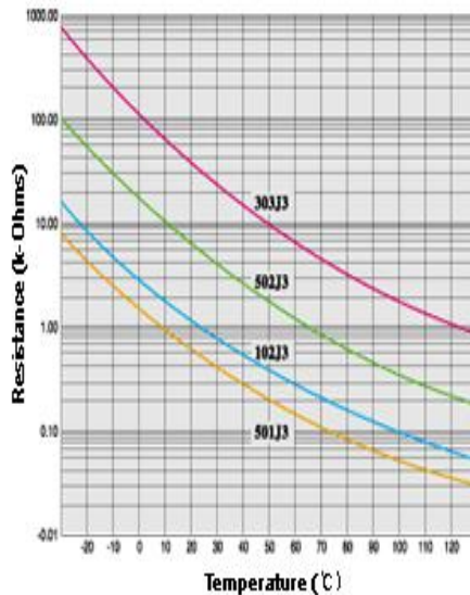
3mm Series
