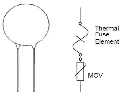
Two-terminal(2A/2B Type)
