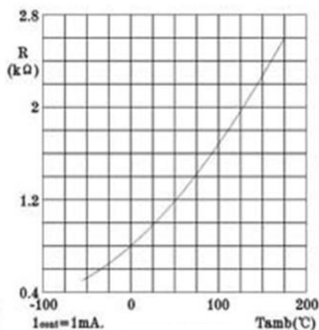
KTY83 Series
