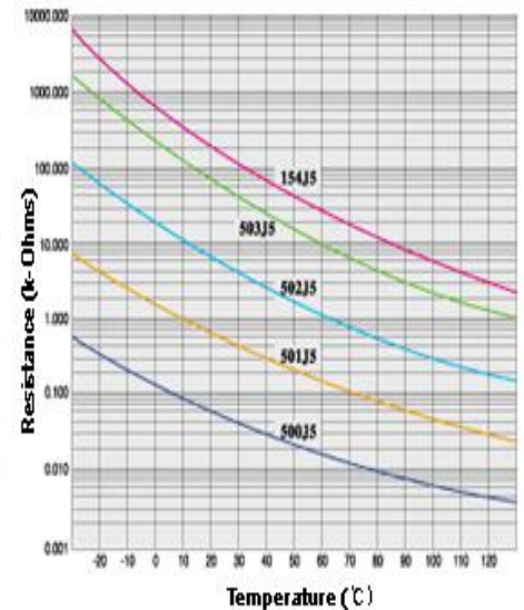
5mm Series
